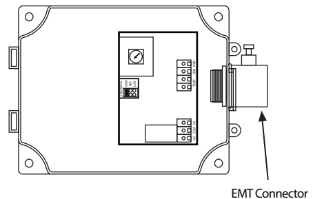
EMT Connector
