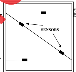
PLACEMENT OF A 12' FLEX-DUCT SENSOR IN A 48" SQUARE DUCT
