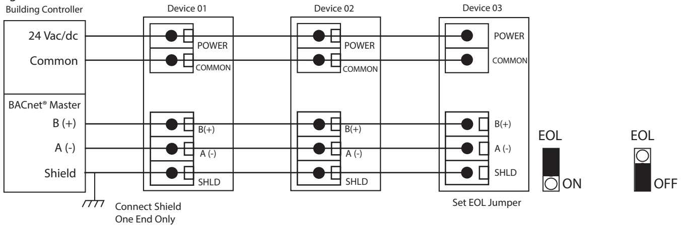
Figure 7 Building Controller
