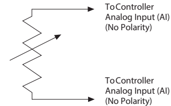
Figure 3 2 Wire Termination for Thermistor or RTD
