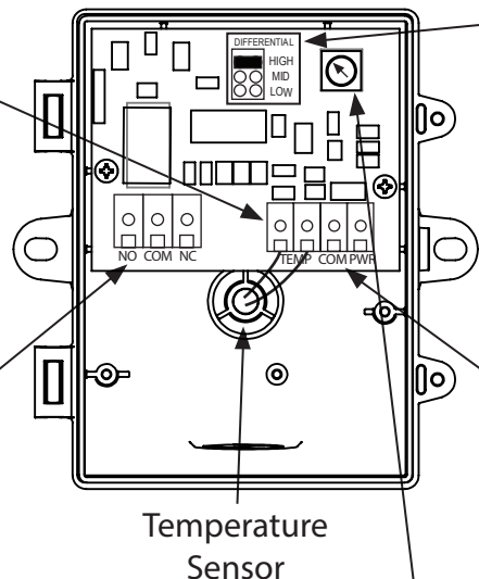
Figure 10 Setpoint Adjustment
