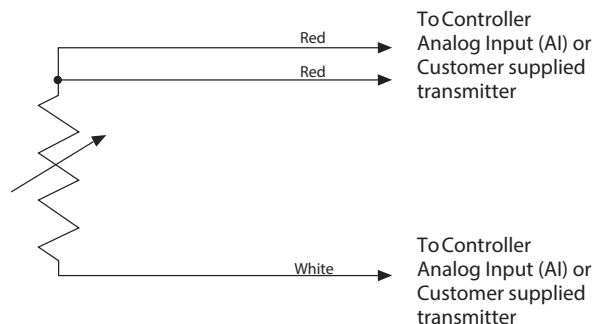
3 Wire Termination
