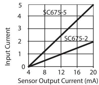
SC-675-2/5 Factory Calibrated Ranges
