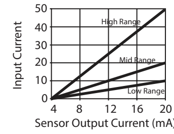
SC-675-R1 Factory Calibrated Ranges SC-675-R2 Factory Calibrated Ranges
