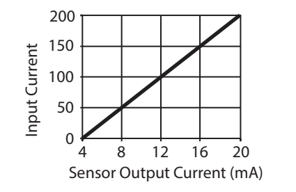
SC-675-200 Factory Calibrated Range
