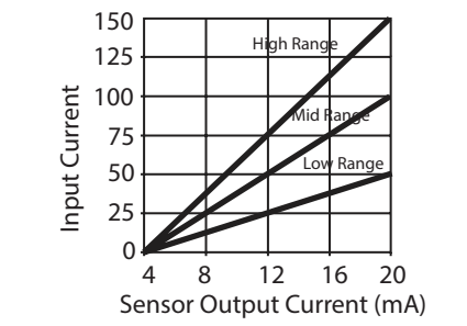
SC-675-R1 Factory Calibrated Ranges SC-675-R2 Factory Calibrated Ranges
