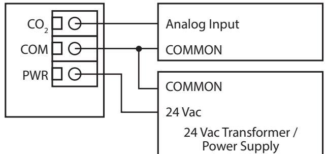
Figure 6 Wiring for all output and external 24 Vac power transformer or external 24 Vac power supply
