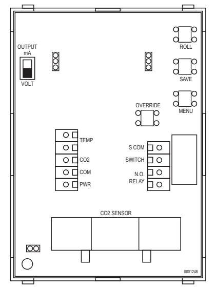
Figure 6 Wiring for all output and external 24 Vac power transformer or external 24 Vac power supply
