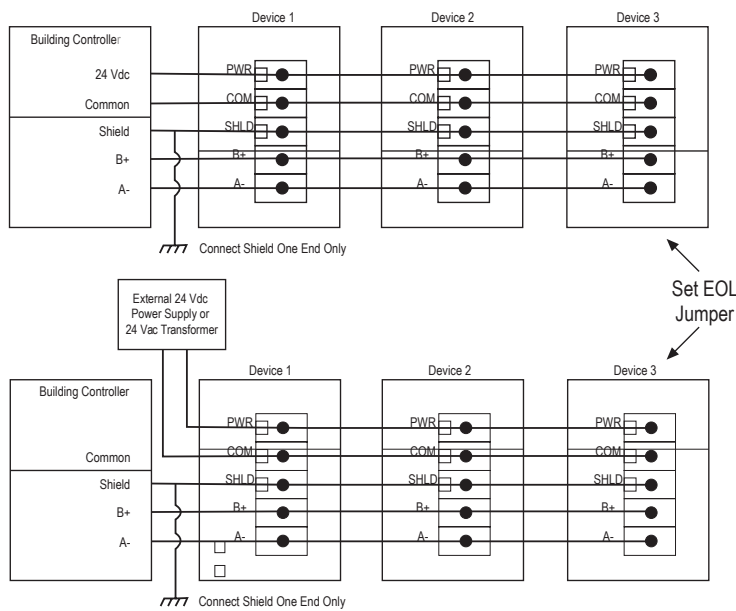
Figure 11 COMMUNICATION WIRING
