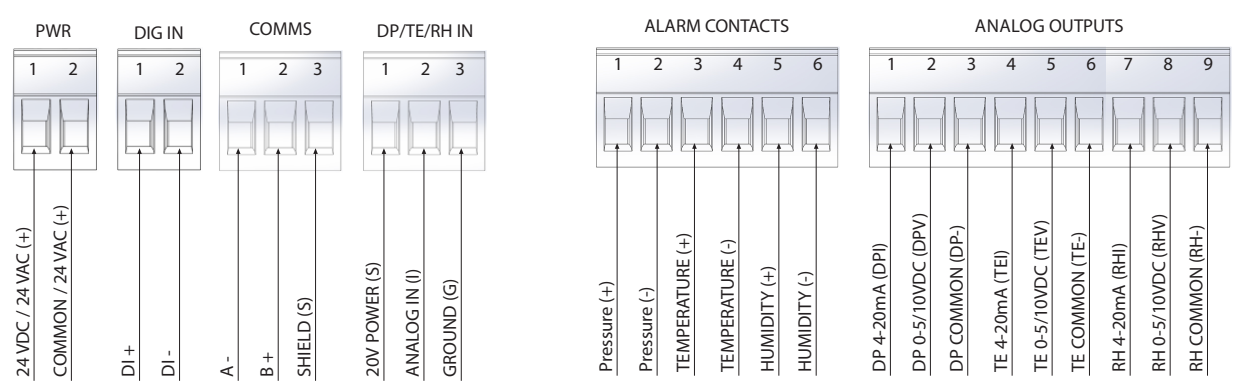
Figure 12 CONNECTORS (Front view, screw on top)
