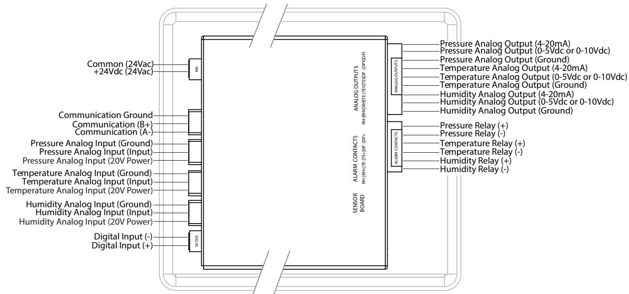
Figure 9 REAR VIEW
