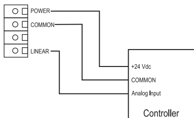
Typical wiring for 24 Vdc power from controller
