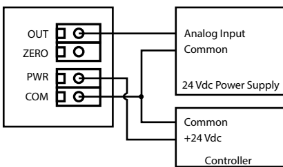
Wiring all output signals and external 24 Vdc power supply
