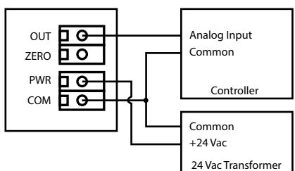
Wiring all output signals and external 24 Vac power supply
