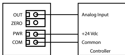
Wiring all output signals and 24 Vdc power from controller
