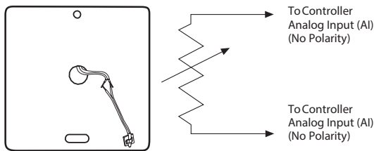
Figure 3 2 Wire Termination for Thermistor or RTD
