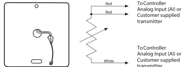
3 Wire Termination for Thermistor or RTD
