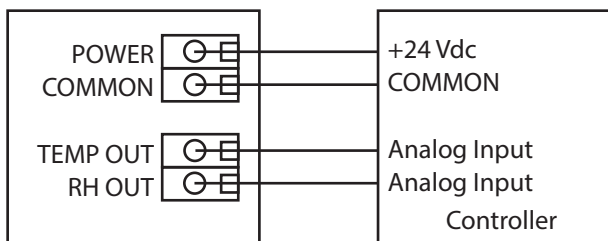
Wiring for voltage output signal for 24 Vdc power from controller
